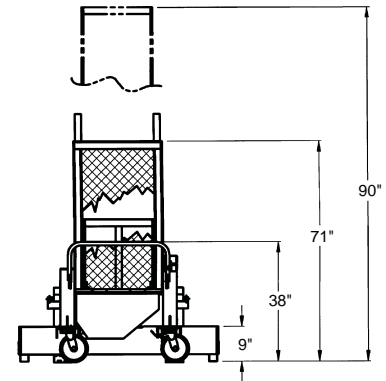
Drawings reflect BPM/BPS-50
