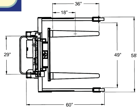
Drawings reflect BPM/BPS-50
